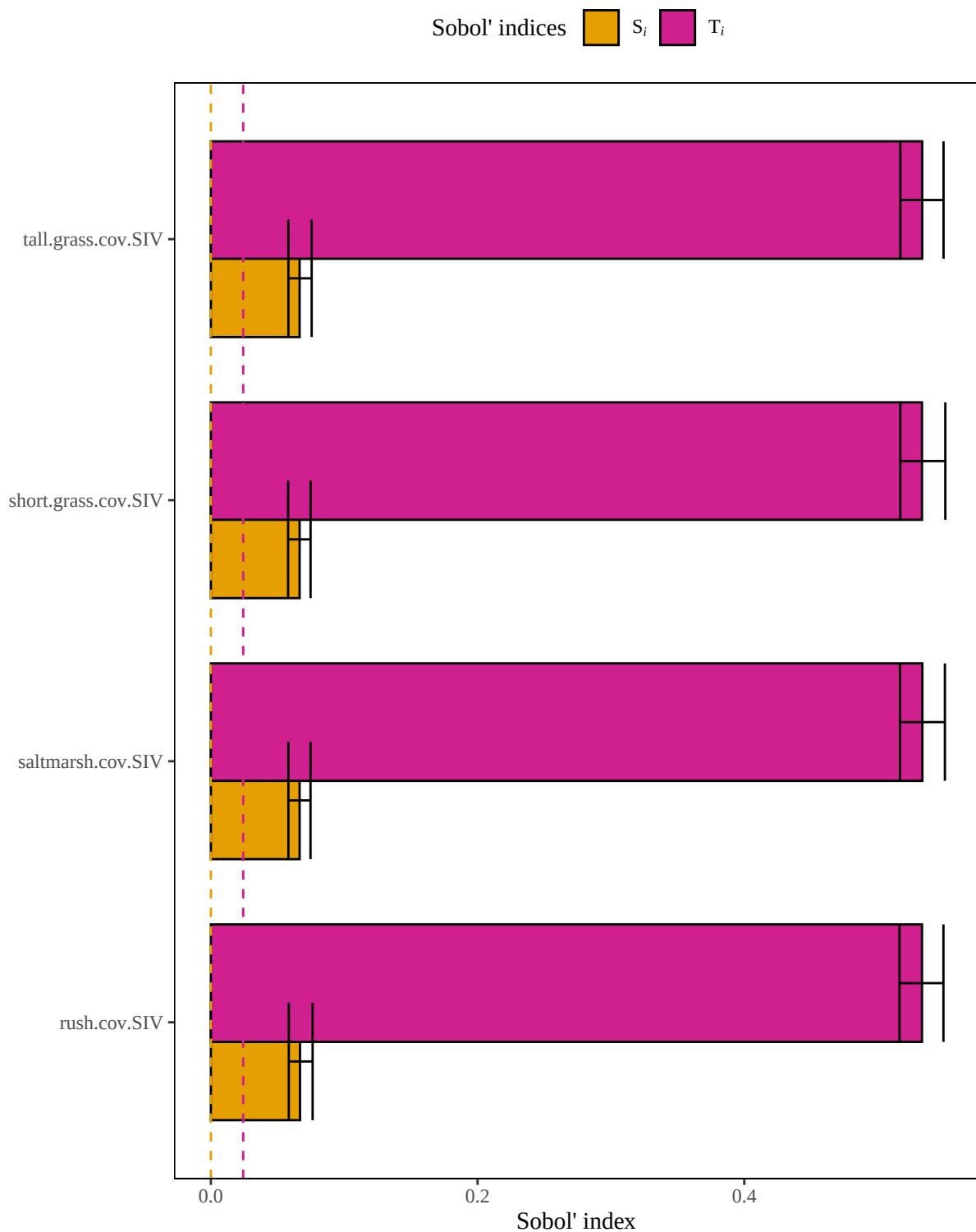
Figure 5. Results of a sensitivity analysis for the blackshoulderedkite model based on a geometric mean structure. Dashed lines represent baseline numerical approximation error for S_i and T_i ( i.e. , dummy variables).
