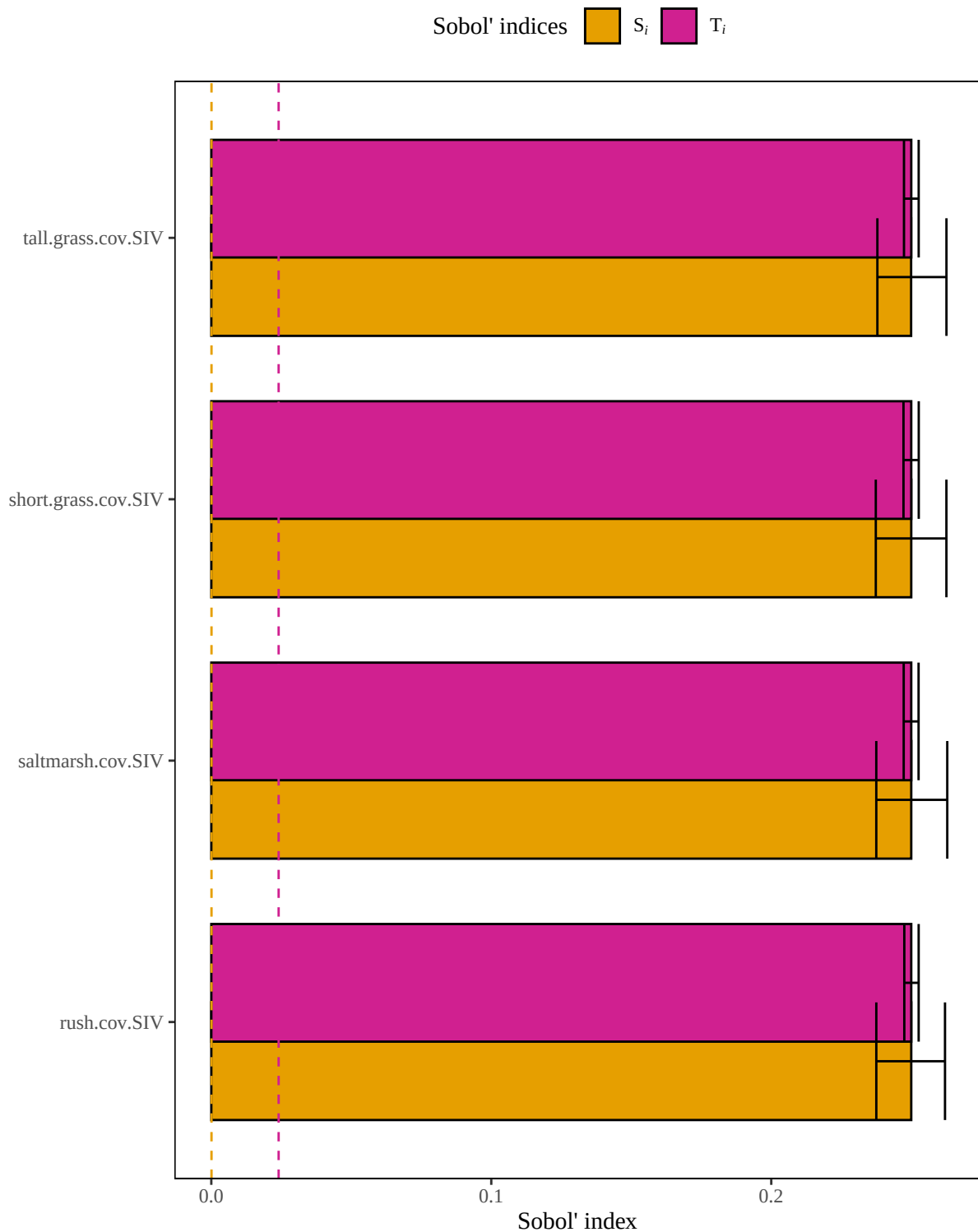
Figure 4. Results of a sensitivity analysis for the blackshoulderedkite model based on an arithmetic mean structure. Dashed lines represent baseline numerical approximation error for S_i and T_i ( i.e. , dummy variables).
